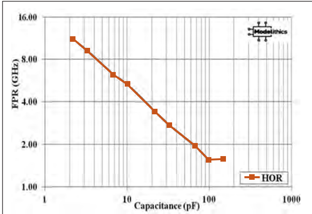
DLC70A Horizontal First Parallel Resonance(FPRs)
